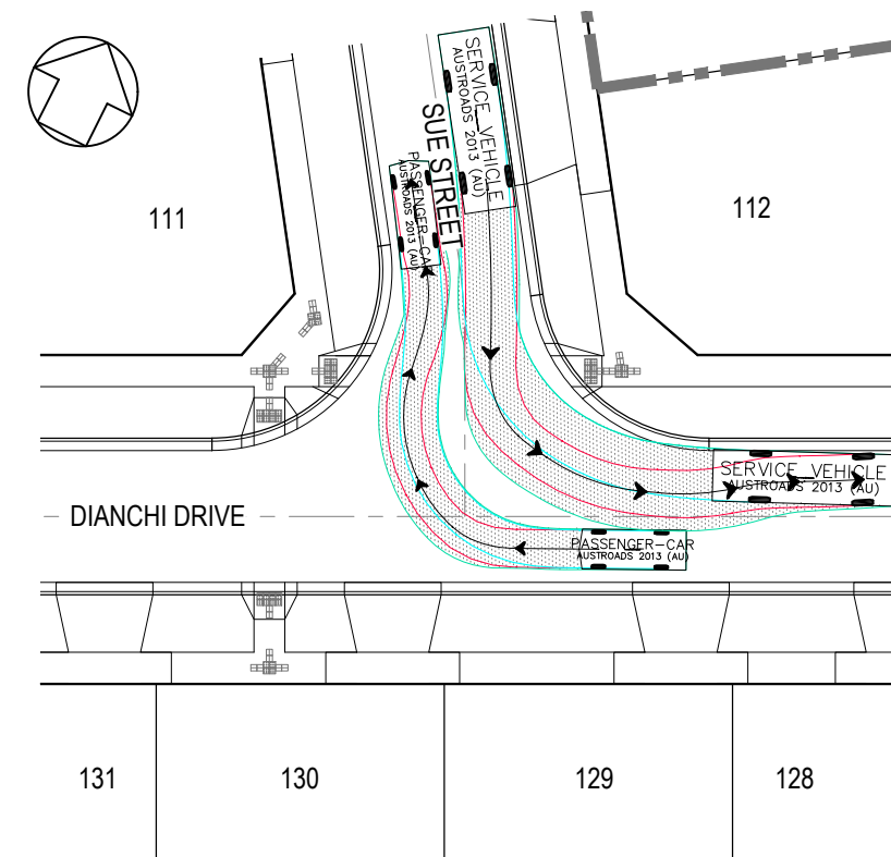
VEHICLE SWEEP PATH DIANCHI DRIVE & SUE STREET
