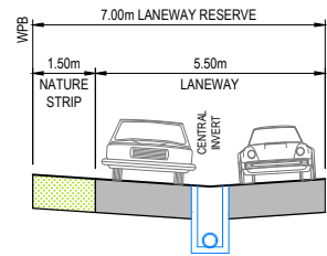
TYPICAL 7.0m LANEWAY
