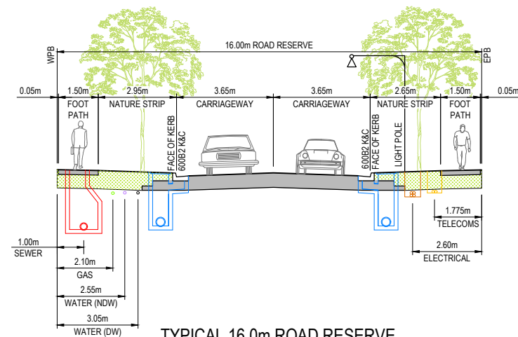
TYPICAL 16.0m ROAD RESERVE
