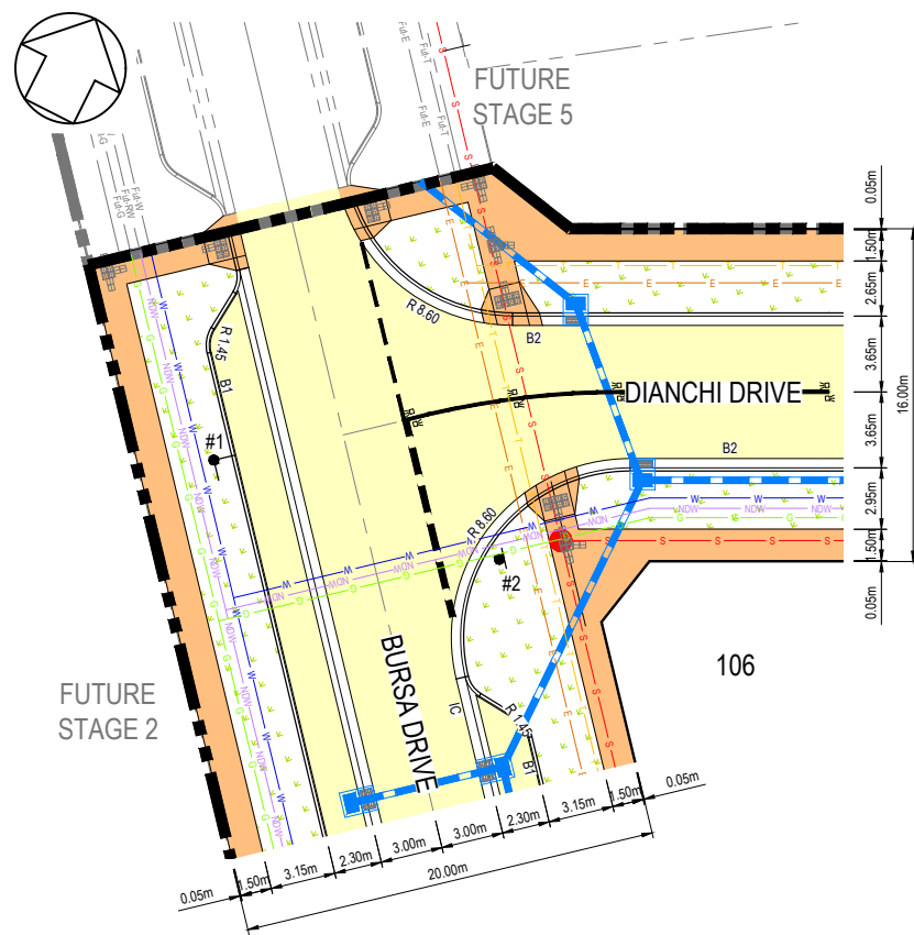
INTERSECTION LAYOUT BURSA DRIVE & DIANCHI DRIVE SCALE 1:200 @ A1
