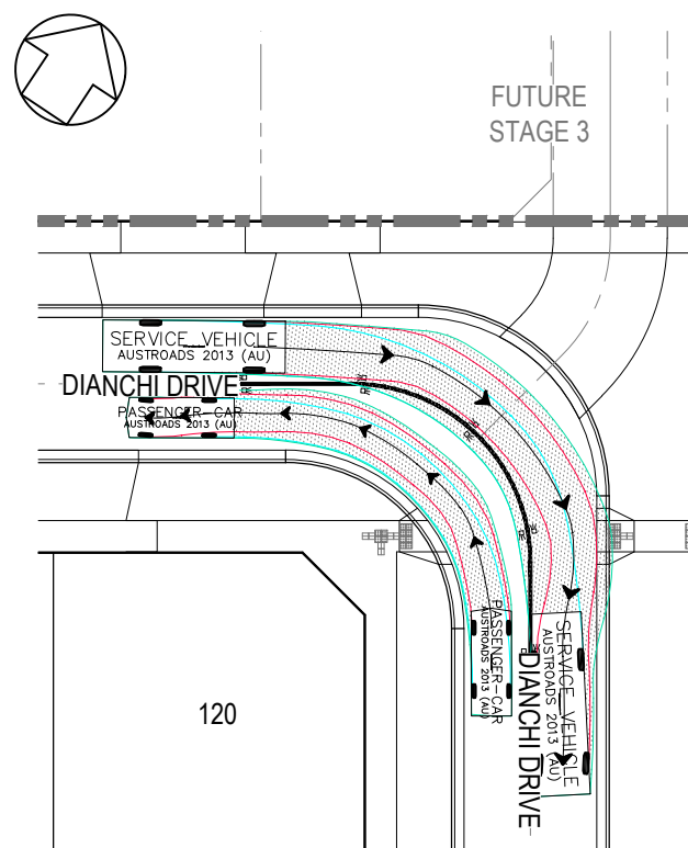
VEHICLE SWEEP PATH DIANCHI DRIVE
