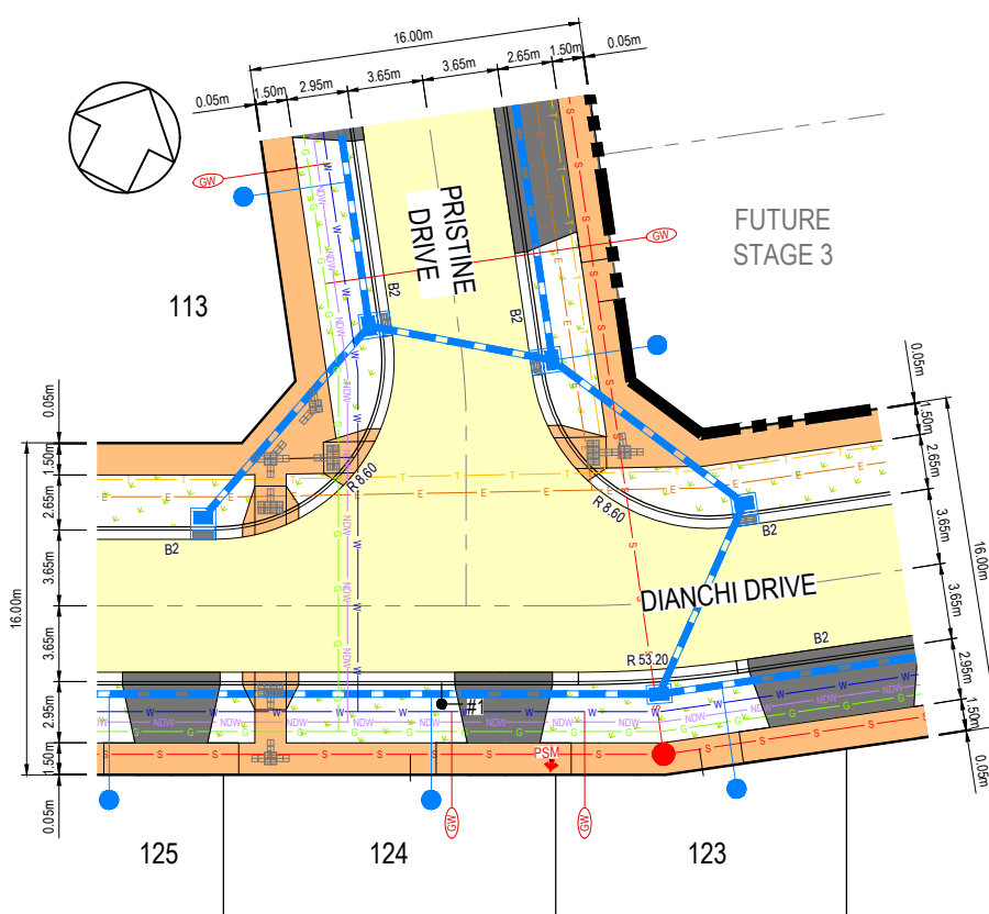
INTERSECTION LAYOUT PRISTINE DRIVE & DIANCHI DRIVE SCALE 1:200 @ A1
