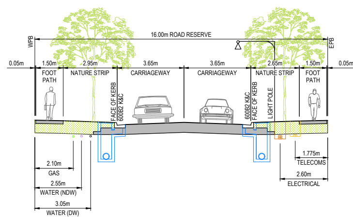
TYPICAL 16.0m ROAD RESERVE
