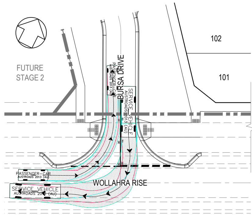
VEHICLE SWEEP PATH BURSA DRIVE & WOLLAHRA RISE SCALE 1:200 @ A1
