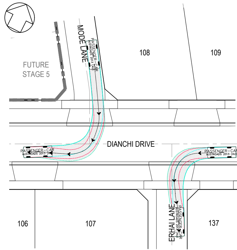
VEHICLE SWEEP PATH DIANCHI DRIVE, MODE LANE & ERHAI LANE SCALE 1:200 @ A1
