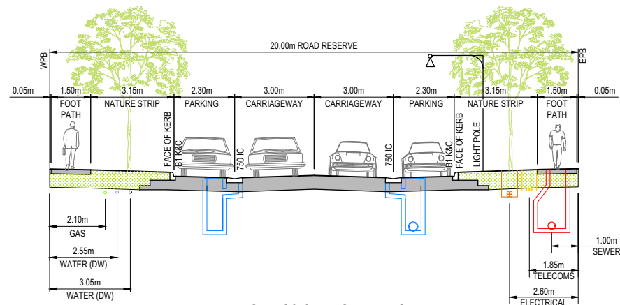
TYPICAL 20.0m ROAD RESERVE
