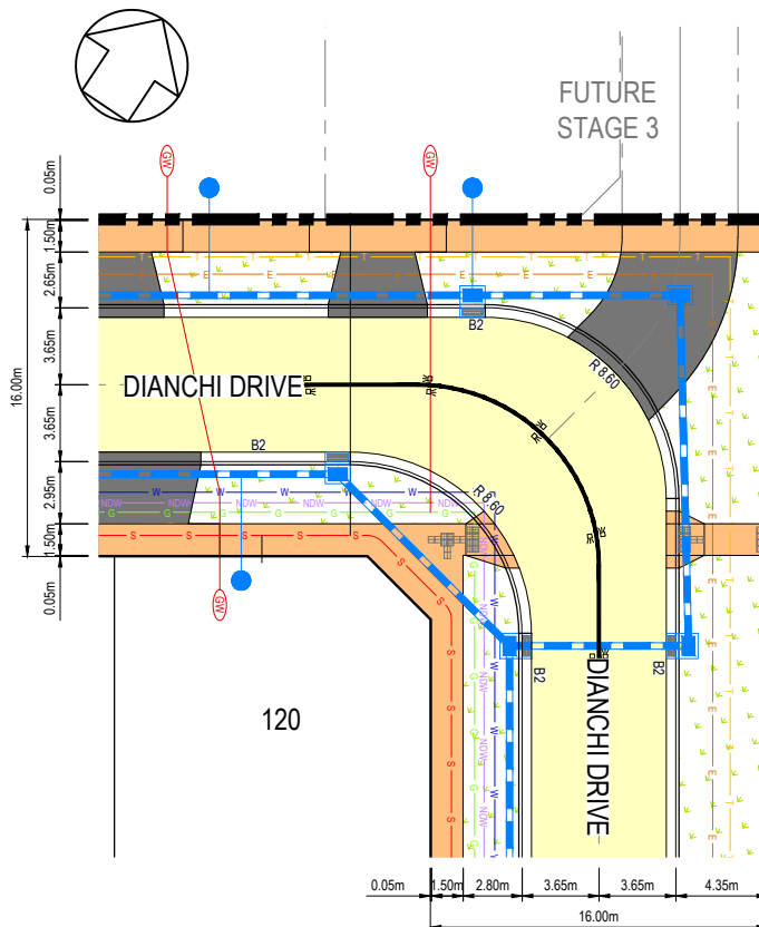
INTERSECTION LAYOUT DIANCHI DRIVE SCALE 1:200 @ A1
