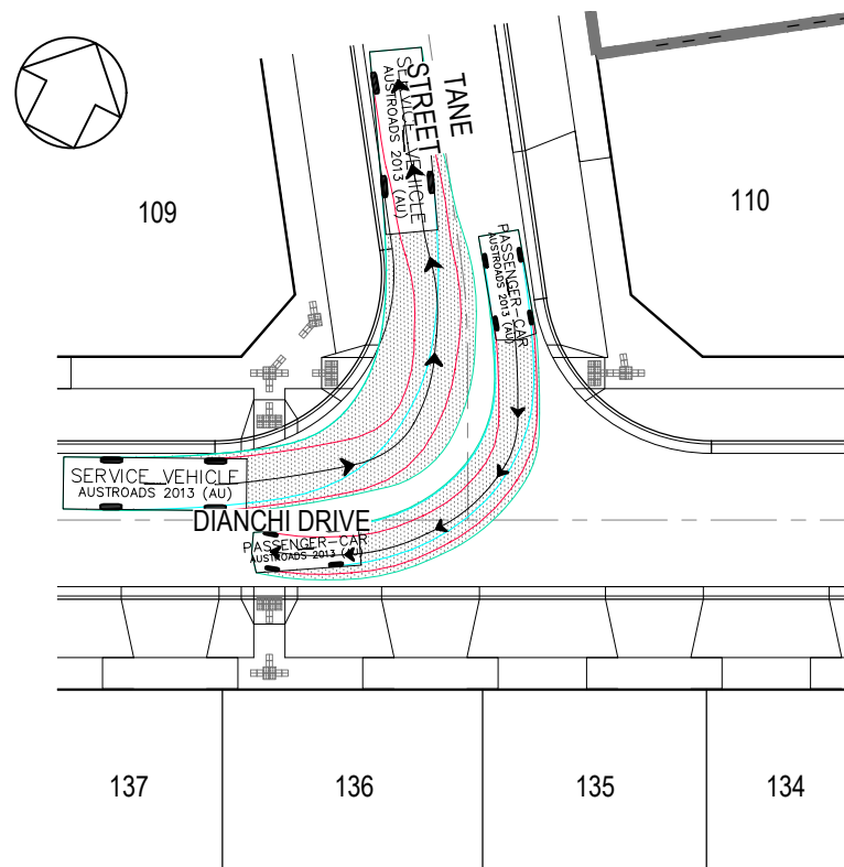
VEHICLE SWEEP PATH DIANCHI DRIVE & TANE STREET
