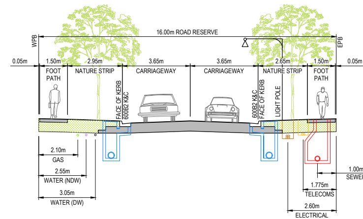
TYPICAL 16.0m ROAD RESERVE
