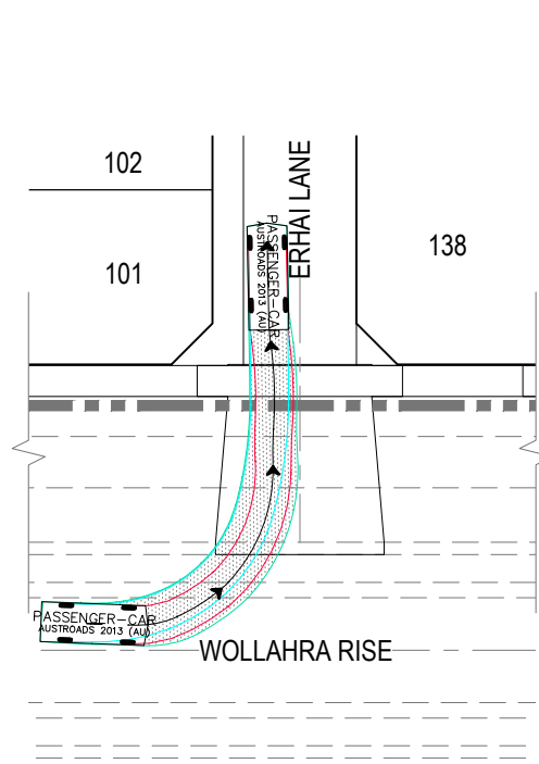
VEHICLE SWEEP PATH ERHAI LANE & WOLLAHRA RISE SCALE 1:200 @ A1
