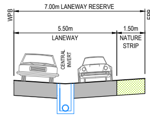
TYPICAL 7.0m LANEWAY
