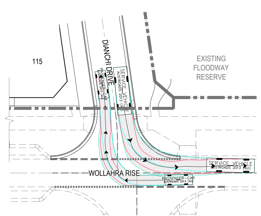
VEHICLE SWEEP PATH DIANCHI DRIVE & WOLLAHRA RISE SCALE 1:200 @ A1
