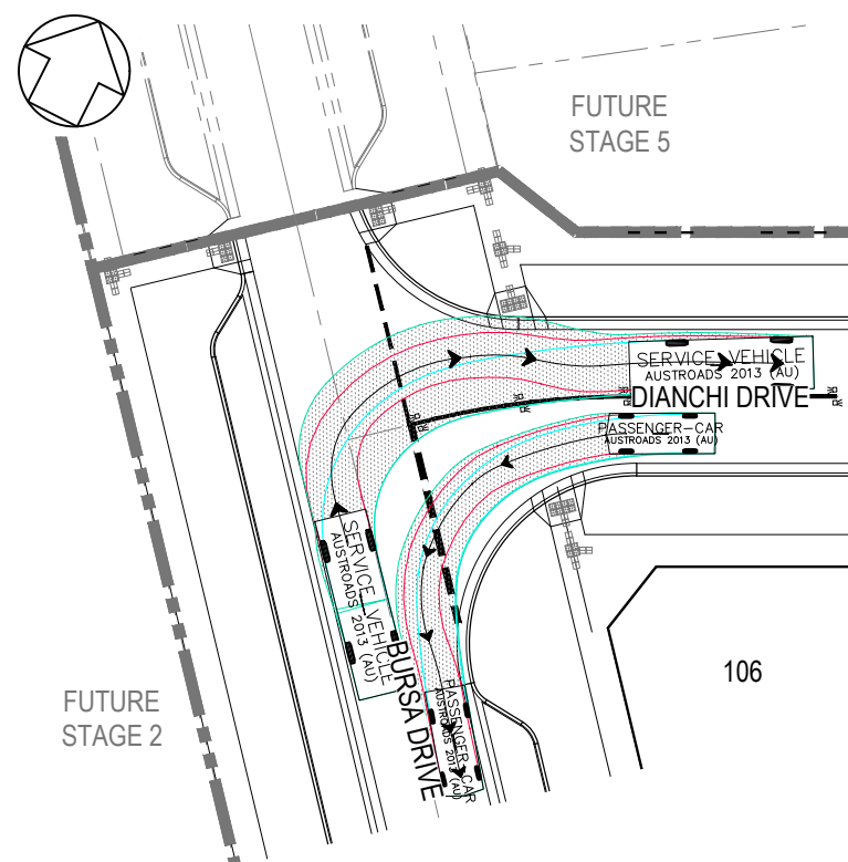
VEHICLE SWEEP PATH BURSA DRIVE & DIANCHI DRIVE
