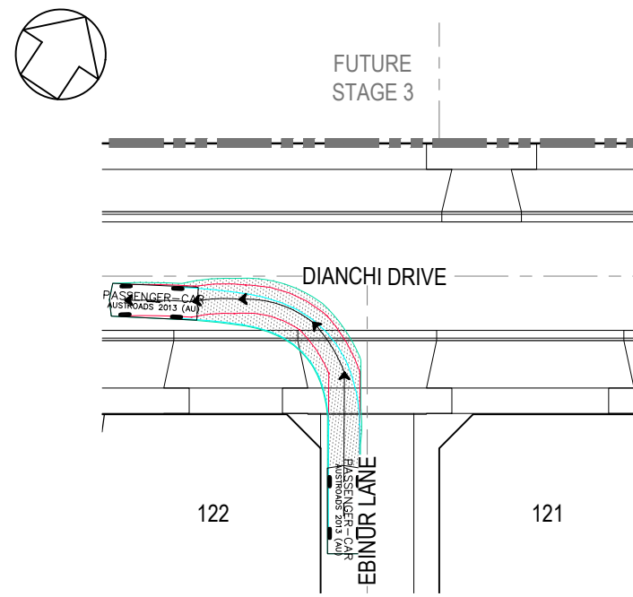
VEHICLE SWEEP PATH DIANCHI DRIVE & EBINUR LANE SCALE 1:200 @ A1
