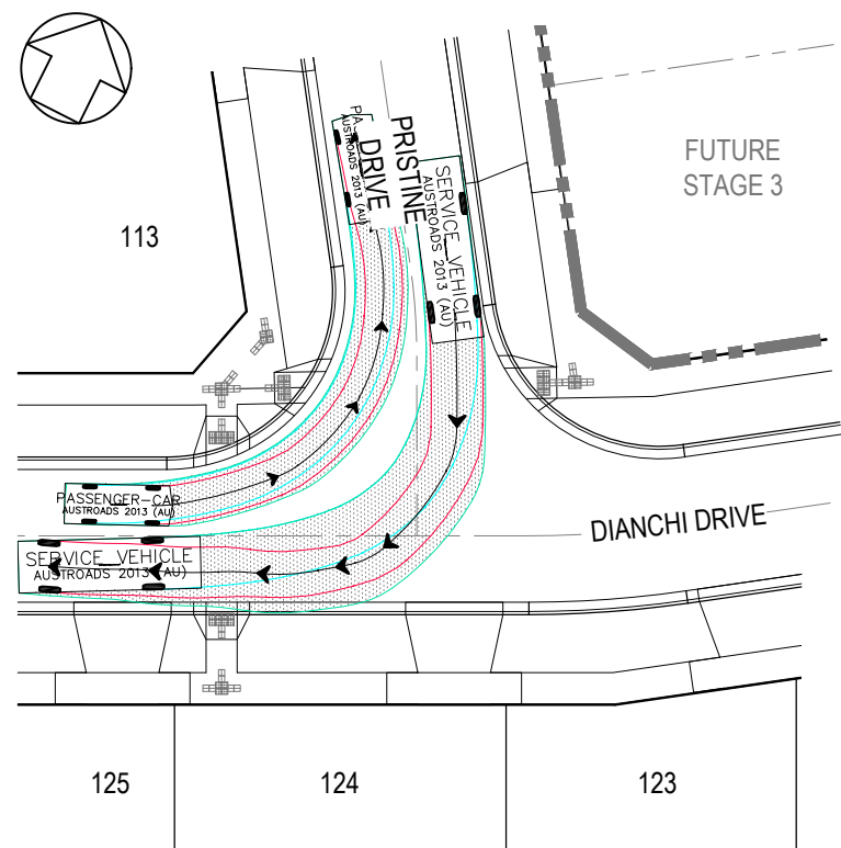
VEHICLE SWEEP PATH PRISTINE DRIVE & DIANCHI DRIVE
