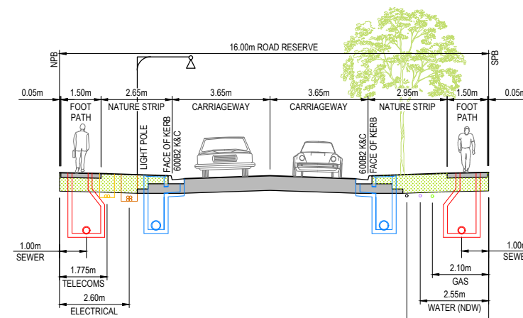
TYPICAL 16.0m ROAD RESERVE
