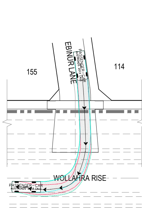
VEHICLE SWEEP PATH EBINUR LANE & WOLLAHRA RISE SCALE 1:200 @ A1
